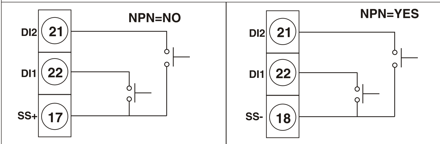
Fig4.DIGITAL INPUT WIRING DIAGRAM
