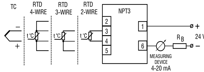
Fig. 2 Electrical connections
